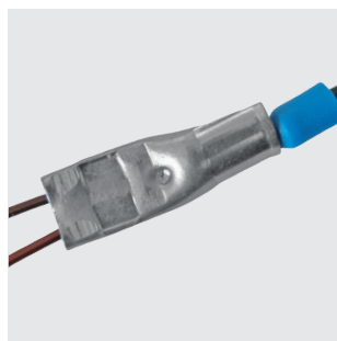
Form of crimping on wire.
