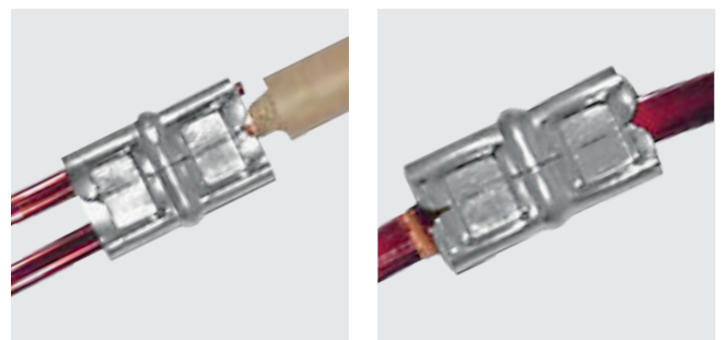
Form of crimping on wire.
